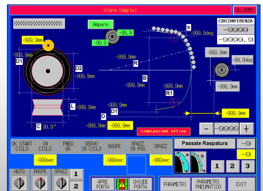
Detail of PLC control panel
